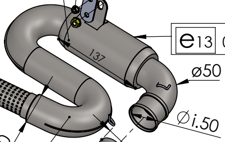
CATALYTIC CONVERTER
