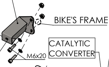
BIKE'S FRAME BIKE'S FRAME BIKE'S FRAME 2x S.s bushing cod.204833 2x Flange cod.204569 e13 00088F
