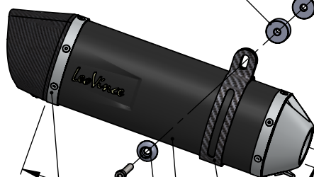
Aluminium spacer ø30X15x8.5 Cod. 206663
