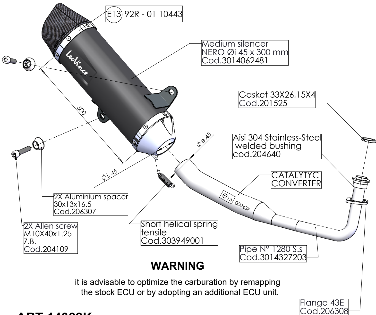
Flange 43E Sp. 5mm Cod. 206308
