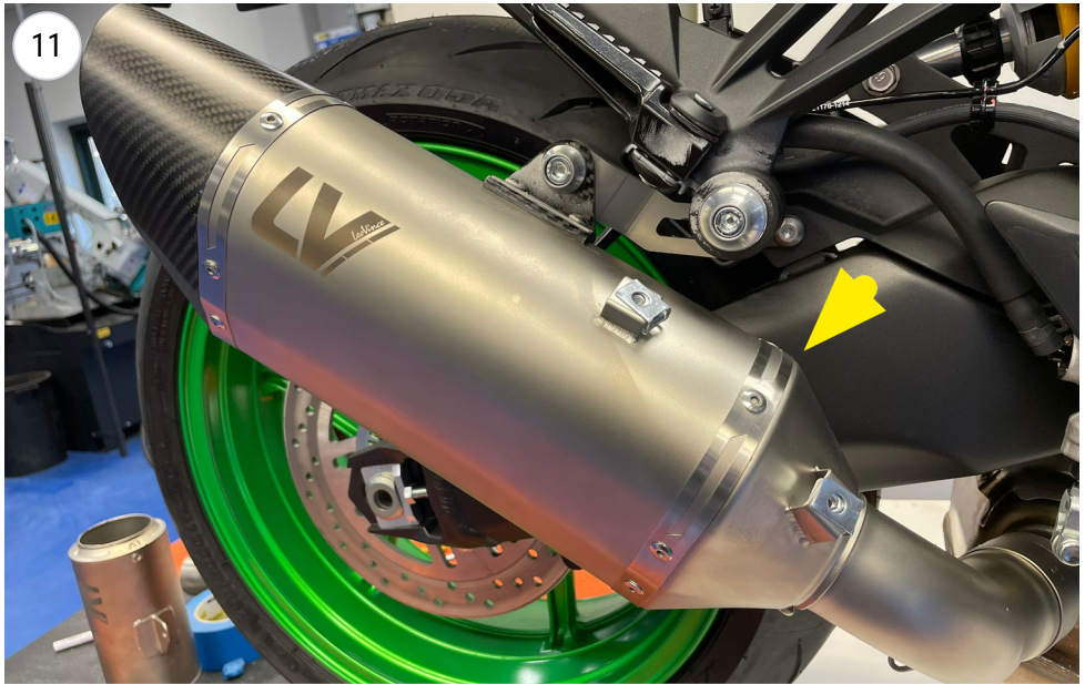
FIT THE MUFFLER AND SCREW - MOUNTING FOR KAWASAKI Z 1100
