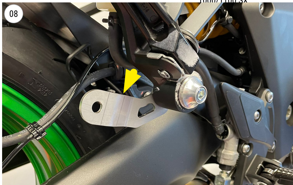
FIT THE LEOVINCE BRACKET - MOUNTING FOR KAWASAKI Z 1100
