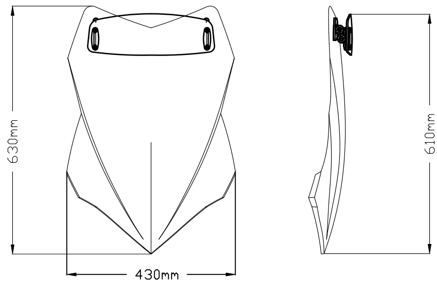
TOURING SCREEN WITH VISOR AT UPPER POSITION
