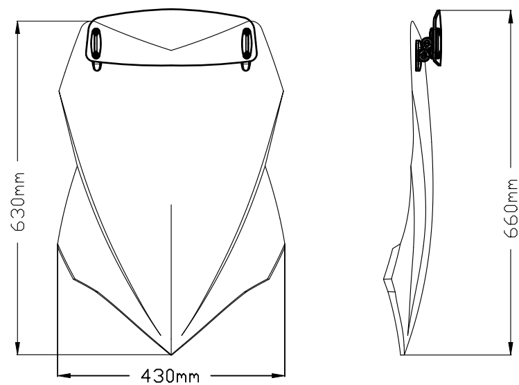
TOURING SCREEN WITH VISOR AT UPPER POSITION
