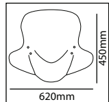
MOD. TOURING
