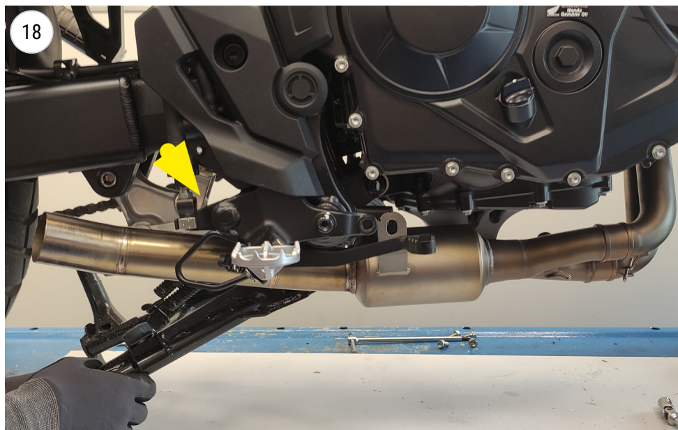
re-install the sonda lambda/O2 sensor
