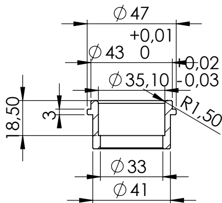
Bushing P/N 204833
