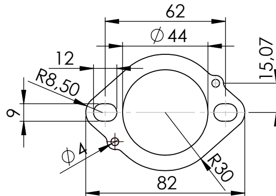
Flange sp. 5mm P/N 204569
