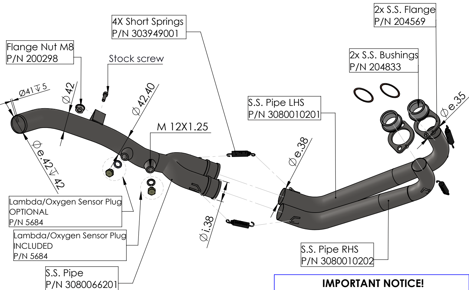
Bushing P/N 204833
