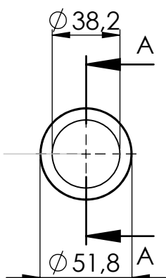
S.S. Bushing P/N 207105
