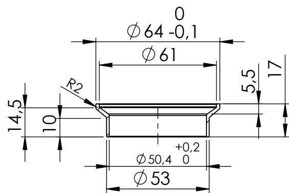
welded bushing
