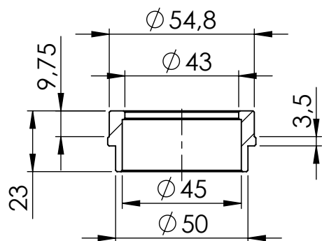
bushing cod.206424R
