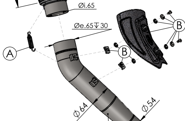
Wool Repack kit P/N 414208R
