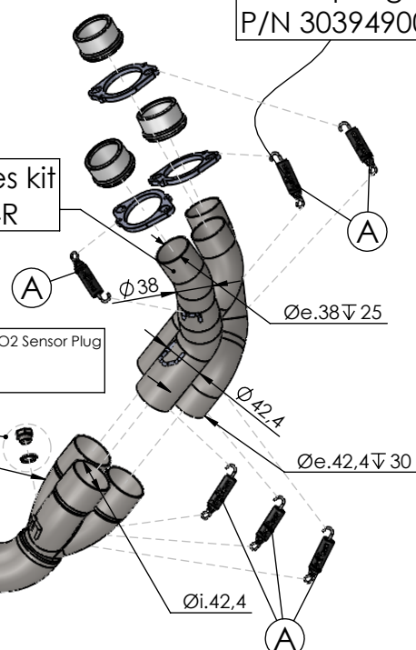
S.S. Secondary Pipe kit P/N 3015638202R
