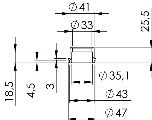
S.S. Bushing P/N 204833
