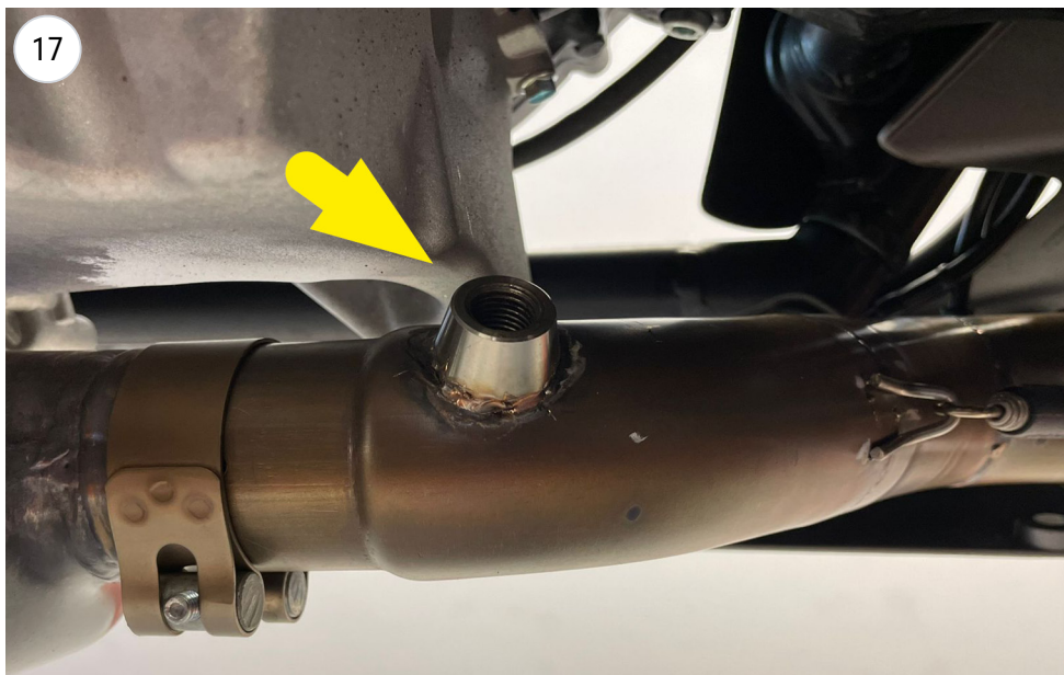
screw the sonda lambda / oxygen sensor
