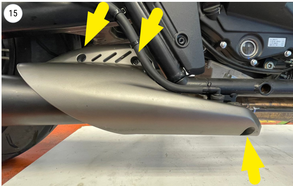
install the heat shield
