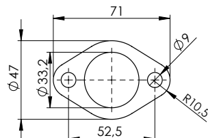
Flange s.s. "43E" cod.206308 sp.5mm
