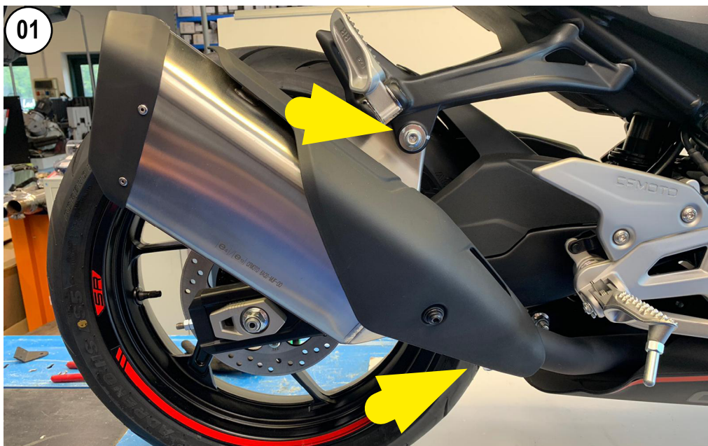
UNSCREW, LOOSE THE CLAMP AND REMOVE THE MUFFLER
