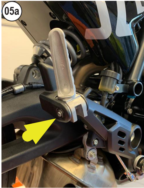
REMOVE THE SEEGER
