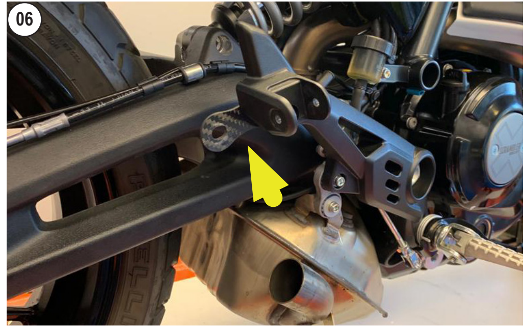
INSTALL THE CARBON BRACKET
