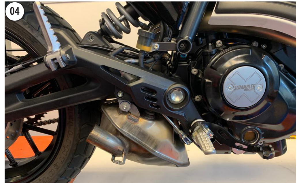
REMOVE THE STOCK MUFFLER
