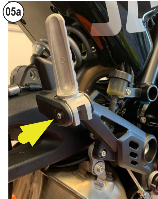
REMOVE THE SEEGER
