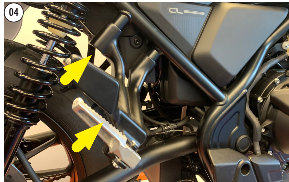
UNSCREW AND REMOVE THE FOOTPEG
