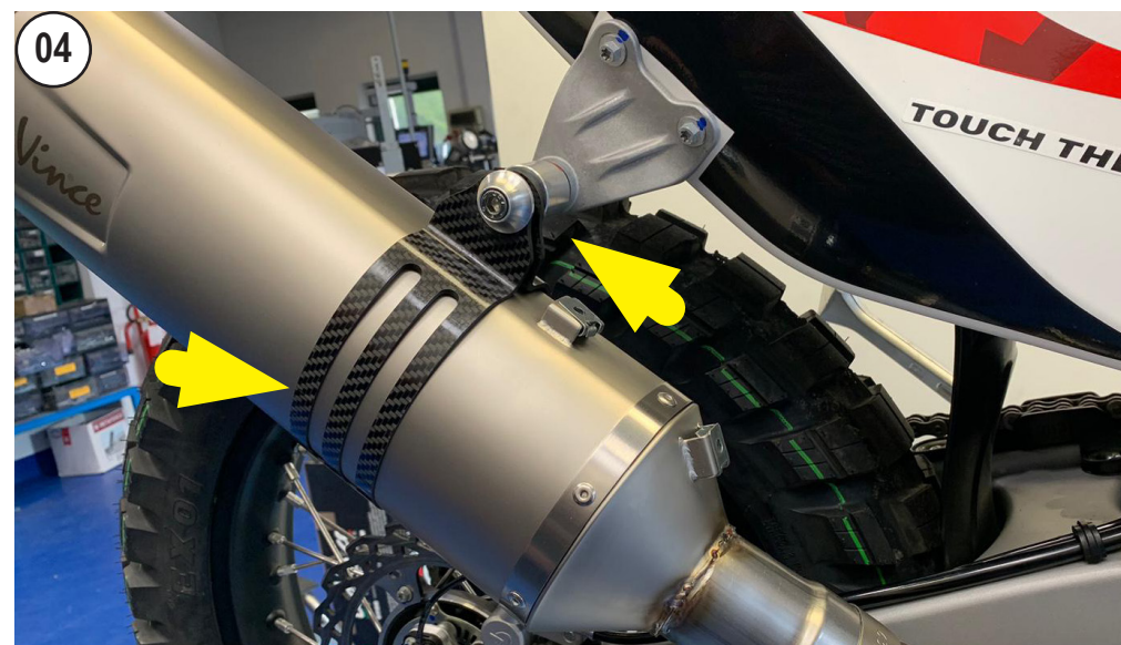
FIT THE CLAMP TO THE LEOVINCE MUFFLER AND MOUNT SPACERS, WASHERS AS SHOWN ON THE DRAWING AND THEN SECURE BY TIGHTENING NUTS AND BOLTS, IF PROVIDED, OR STOCK (SHOWN ON DRAWING) .
