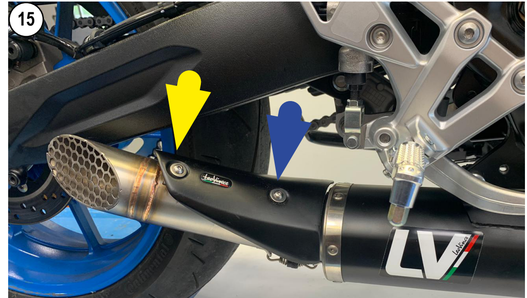
PUT THE CARBON HEAT SHIELD AND SCREW (SEE THE TECHNICAL DRAWING FOR HEAT SHIELD STACKING)
