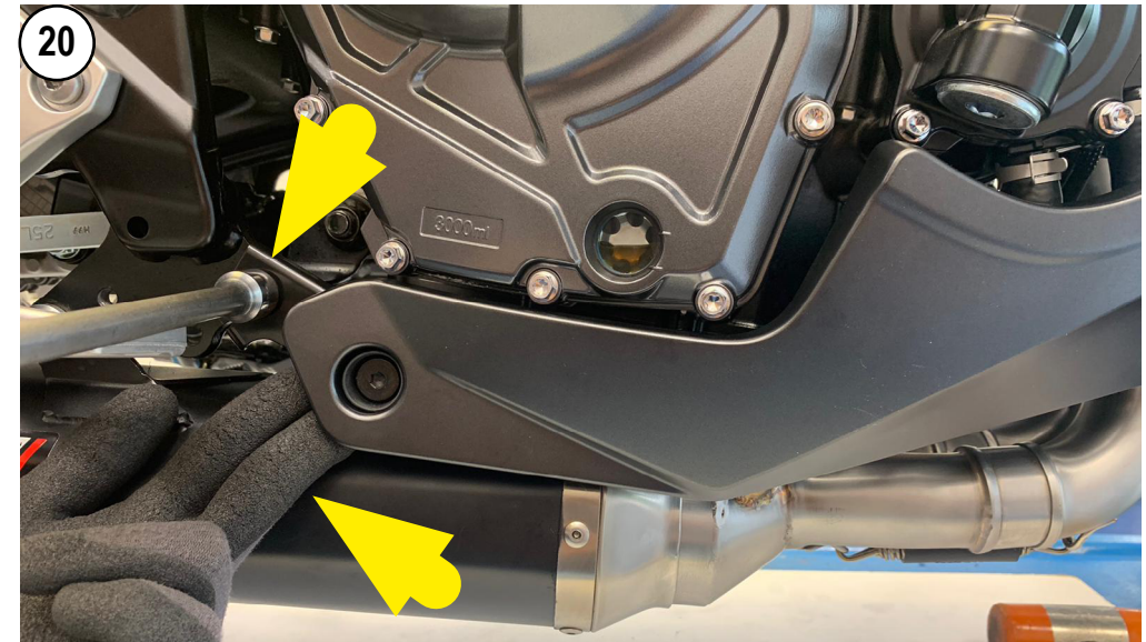
WHEN YOU SCREW THE BRACKET USE YOUR FINGER FOR PUSH UP THE UNDER COWL OTHERWISE THE BRACKET IMPACT ON THE MUFFLER
