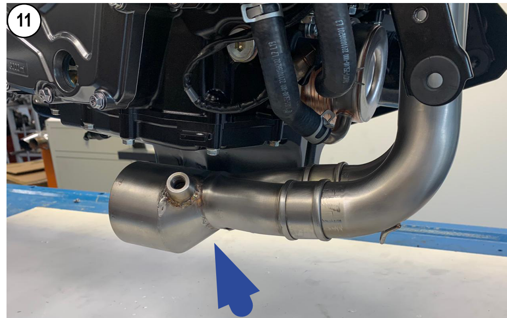
SLIDE IN THE SECONDARY PIPE
