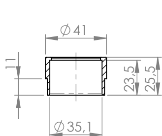
Bushing Cod.206060
