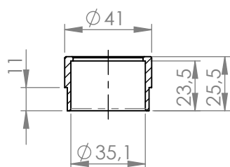
Bushing Cod.206060
