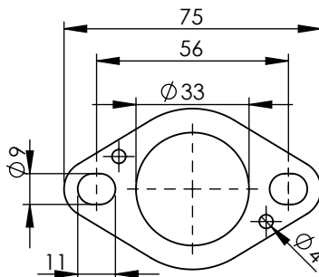
Flange s.s. "45E" cod.205267 sp.6mm
