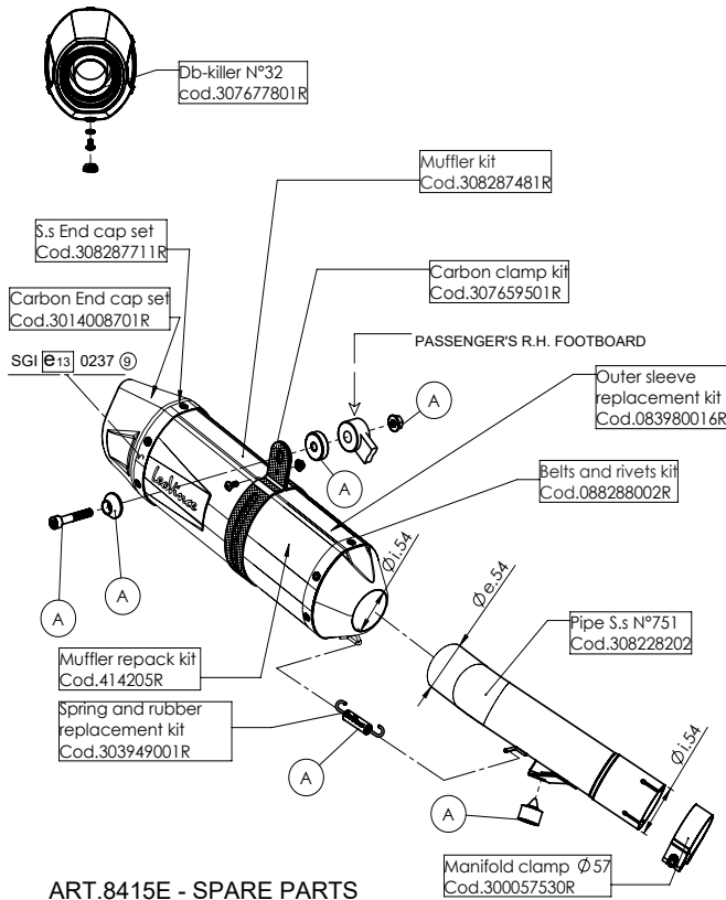
ART.8415E - SPARE PARTS
