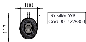
LV ONE EVO silencer RHS carbon fiber
