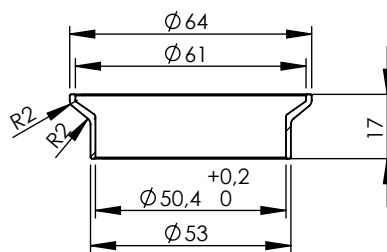
Bushing s.s. cod.206079
