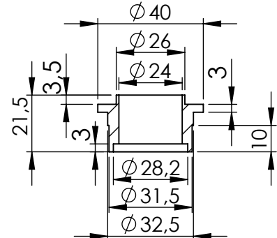
Bushing s.s. cod.206283
