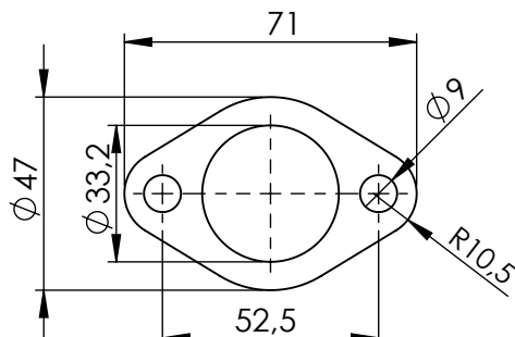
Flange s.s. "43E" cod.206308 sp.5mm
