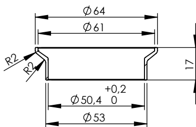
Bushing s.s. cod.206079
