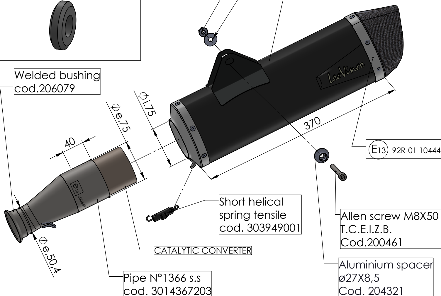
NERO silencer RHS stainless steel black Cod.3014072482
